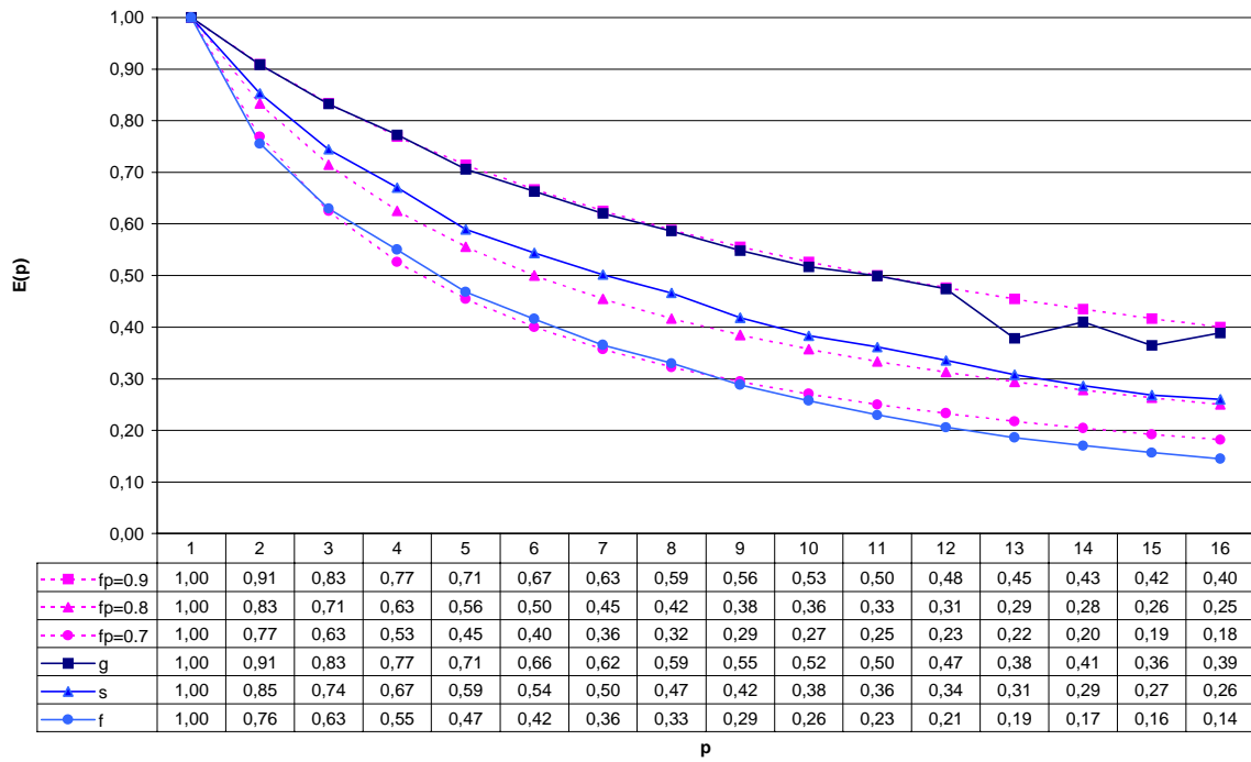
Figure 2 - Father, Son, Grandson and theoretical Amdhal's efficiencies for f_p=0.7 , f_p=0.8 , f_p=0.9
