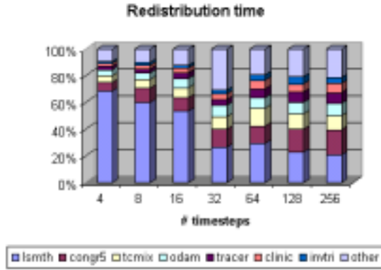
Figure 1 – Time redistribution between M.O.M. subroutines varying the number of timesteps
