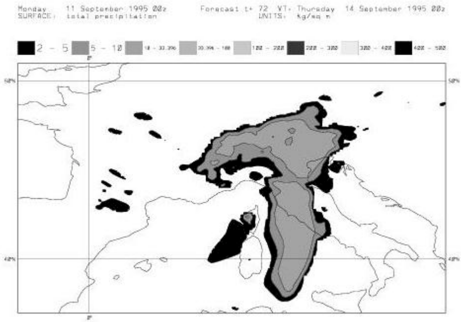
Figure 5 – Total precipitation 72 hours forecast 64 bit numerical representation
