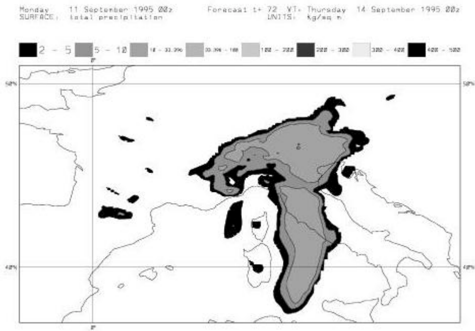
Figure 4 – Total precipitation 72 hours forecast 32 bit numerical representation
