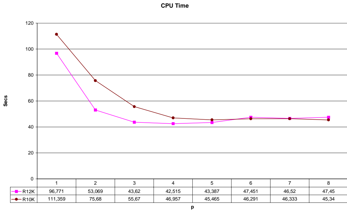
Figure 3 – W.A.M. cpu Time on R12K and R10K
